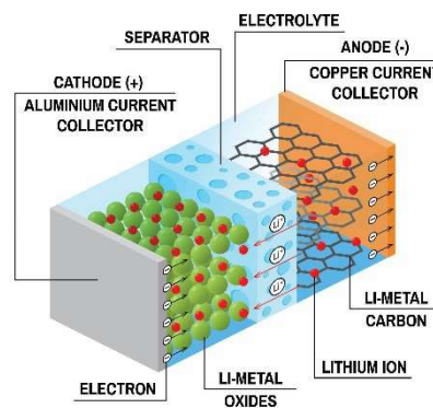
Image 3. Lithium-Ion Cell Discharging Source/Copyright: iStock
